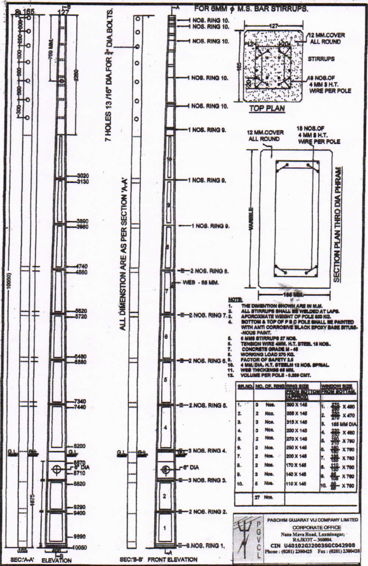
DRAWING OF 10MT x 270 KG PSC POLE
