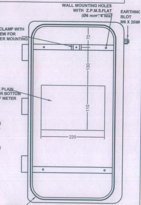
DOOR OPEN VIEW
