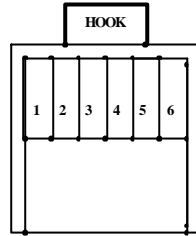
RJ11(HOOK UNDERNEATH)
