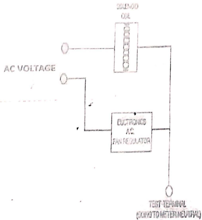
CIRCUIT DIAGRAM FOR TEST JIG TO INTRODUCE CHOPPED A.C. IN NEUTRAL.
