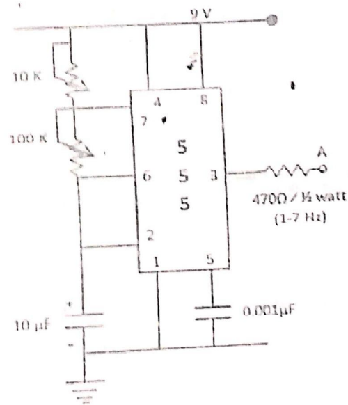
CIRCUIT DIAGRAM FOR DC PULSATING SIGNALS IN NEUTRAL
